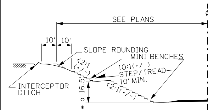
CUT SLOPES - 2:1 OR STEEPER (SEE NOTE NO. 3)
