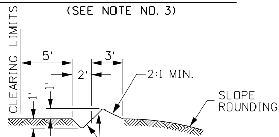
INTERCEPTOR DITCH (SEE NOTE NO. 8)
