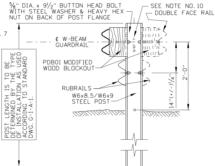
MEDIAN BARRIER DETAIL
