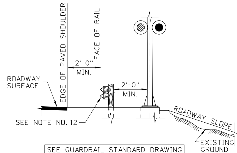
TYPICAL SECTION (WITH GUARDRAIL)
