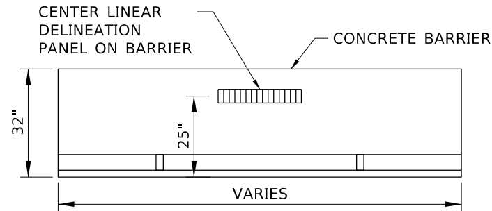
4" x 34" PANEL PLACEMENT ON CONCRETE BARRIER DETAIL
