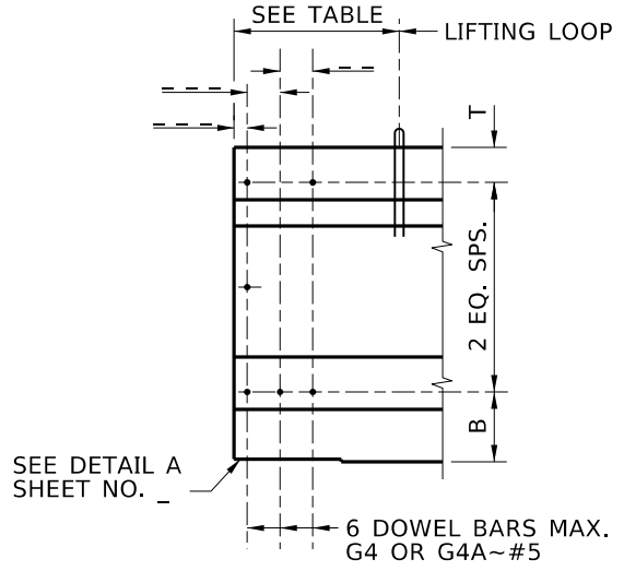
ELEVATION TYPE A EXPANSION
