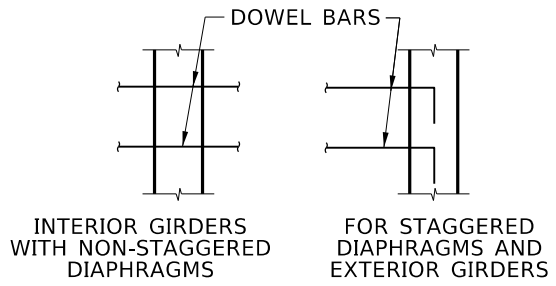
INTERMEDIATE DIAPHRAGM DOWEL DETAILS 1/4"=1'-0"
