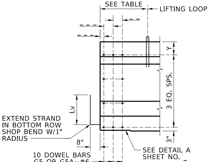
ELEVATION TYPE B FIXED
