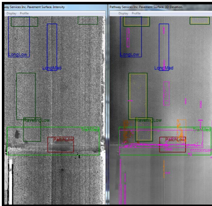
FIGURE 24: AUTO CLASSIFICATION & AUTO CRACK
