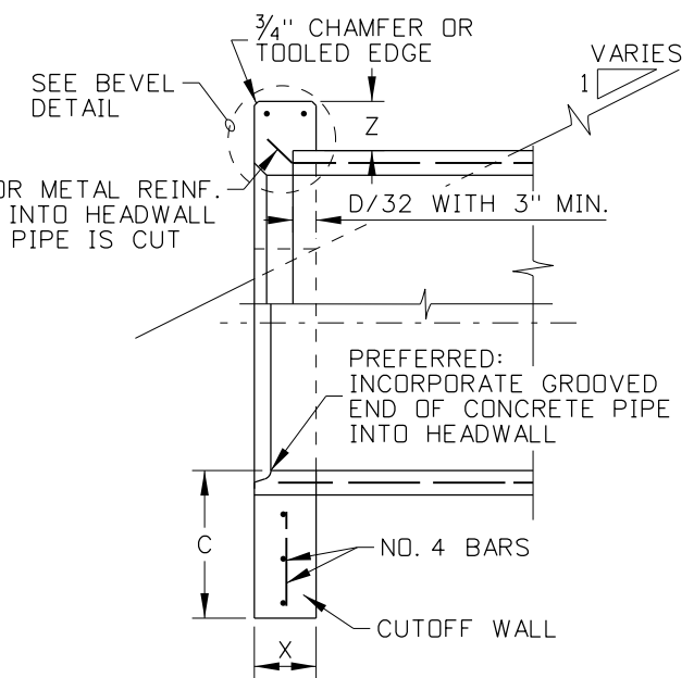
INLET STRUCTURE (CULVERT SIZES 36" TO 180" DIA.)
