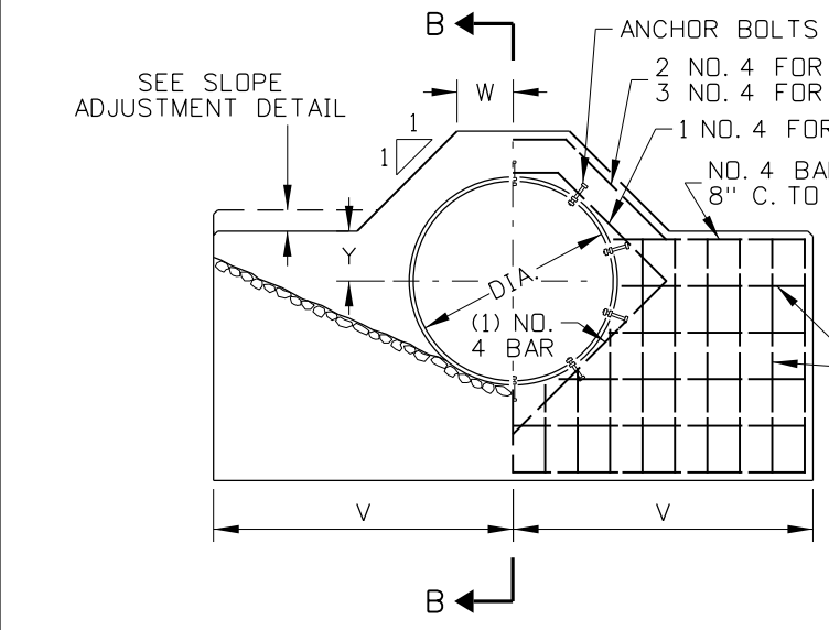
INLET STRUCTURE (CULVERT SIZES 18" TO LESS THAN 36" DIA.)
