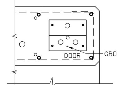
VERIFY PLACEMENT OF 5/8" X 6" X 2" ANCHOR BOLTS ALTERNATE SERVICE PEDESTAL LOCATION (TO BE APPROVED BY ENGINEER)
