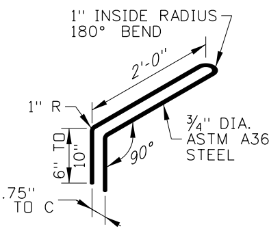
STEEL LOOP BAR DETAIL
