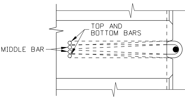
STEEL LOOP BAR PLACEMENT DETAIL
