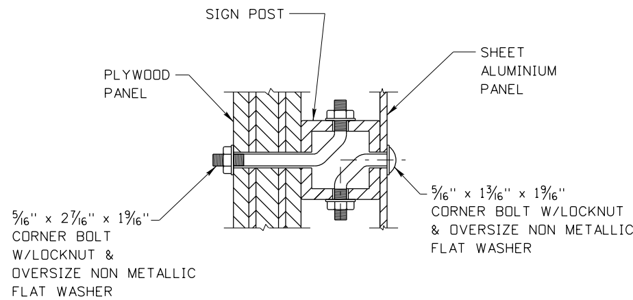
BACK TO BACK SIGN MOUNTING DETAILS
