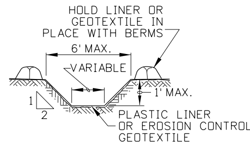
TO BE USED ONLY FOR CLEAR WATER DIVERSION DITCH
