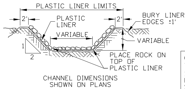
DIVERSION CHANNEL DETAIL
