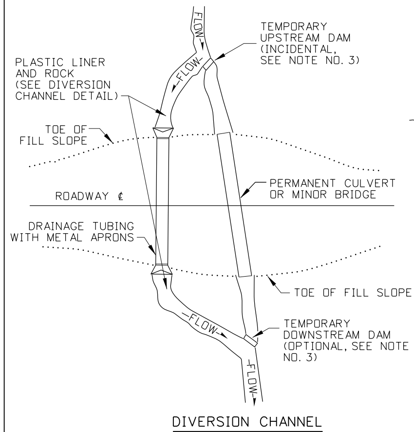
TO BE USED ONLY FOR CLEAR WATER DIVERSION DITCH
