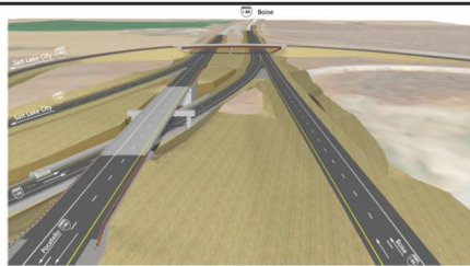
3D Perspective - I-86 WB
