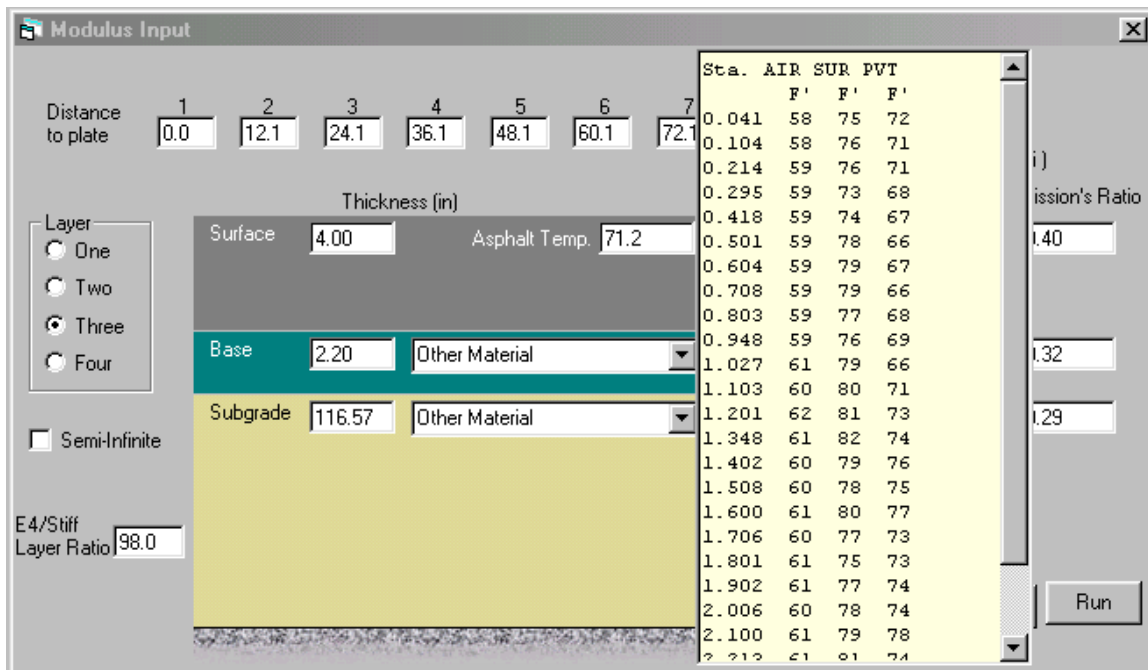
Figure 16. View the FWD Measured Temperature.
