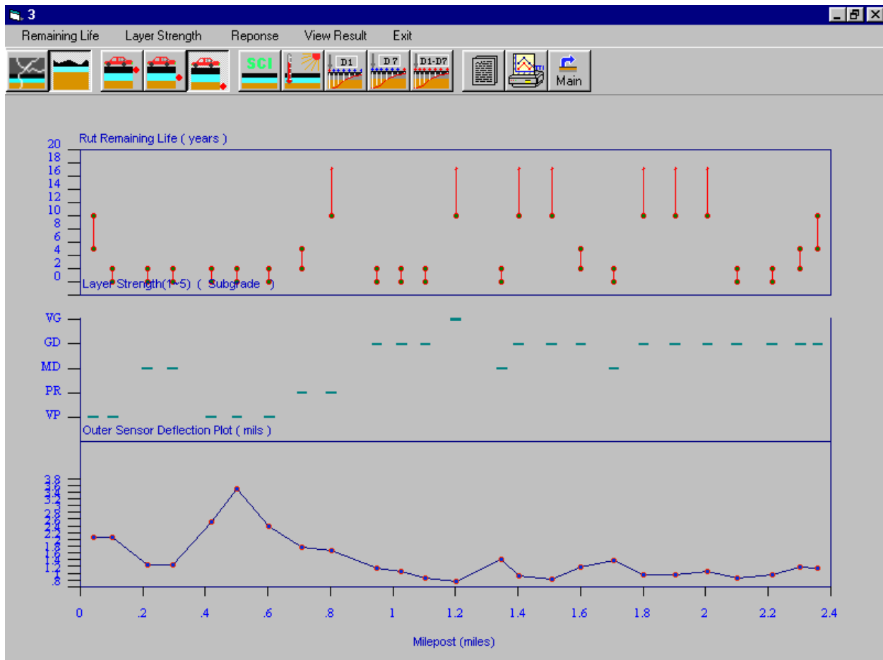
Figure 13. Remaining Life Result Chart.
