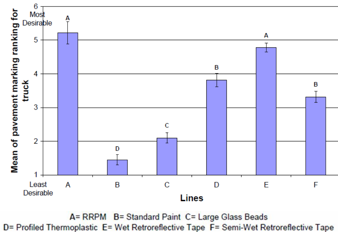
Figure 5. Results of the Preference Ranking of Pavement Markings by Participants for the Wet Truck Condition (22)
