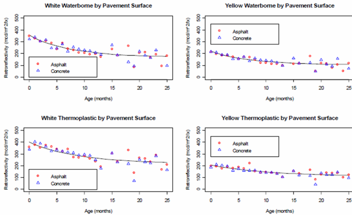
Figure 3. Marking Age by Pavement Surface for White and Yellow Water-borne Paint and Thermoplastics (21)
