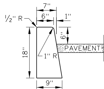
CURB TYPE 2
