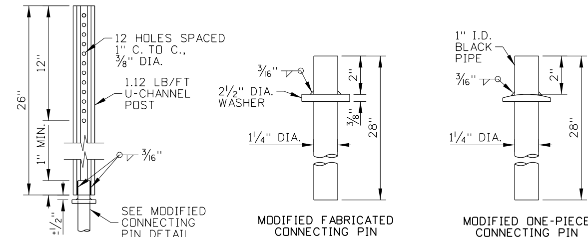
STUB POST FOR USE WITH TYPE 5, 6, 7, OR 8 DELINEATORS MODIFIED FABRICATED CONNECTING PIN MODIFIED ONE-PIECE CONNECTING PIN FOR USE WITH TYPE 5, 6, 7, OR 8 DELINEATORS (SEE STANDARD DRAWINGS G-2-A-1 & G-2-A-2)
