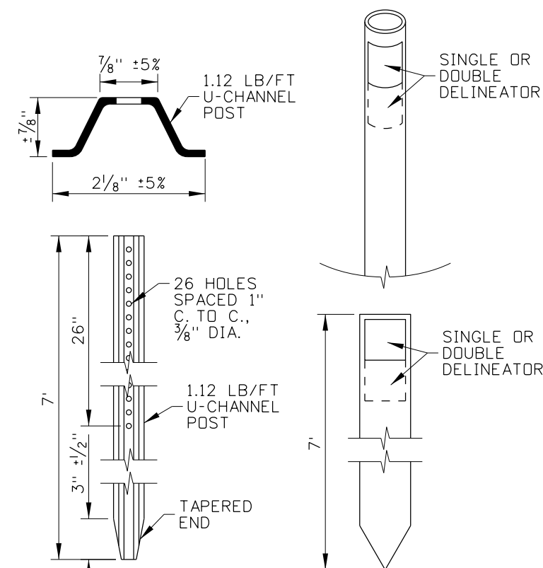
RIGID POST (SEE NOTE NO. 6) FLEXIBLE POST PROPRIETARY POSTS MAY DIFFER FROM THOSE SHOWN (SEE NOTE NO. 6)
